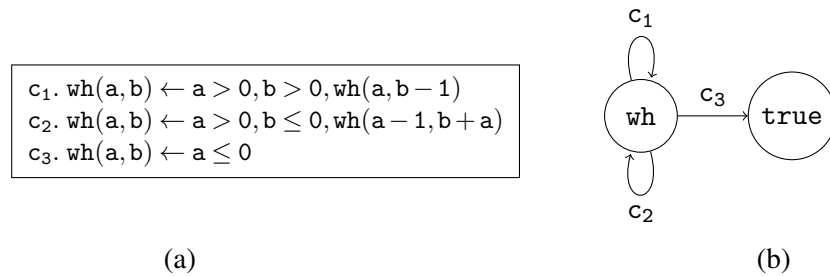
Figure 1: (a) Multi-path loop and (b) its CFG.
